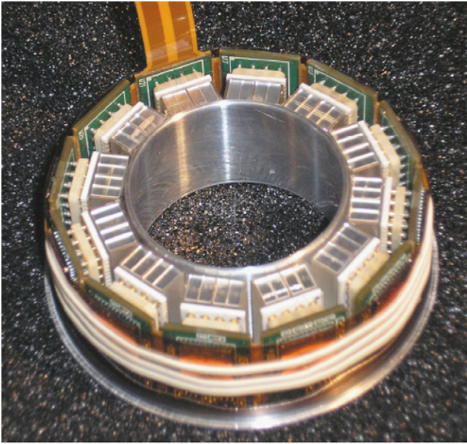
Fig. 1. The RatCAP tomograph consisting of 12 LSO arrays with APDs and associated readout electronics.
