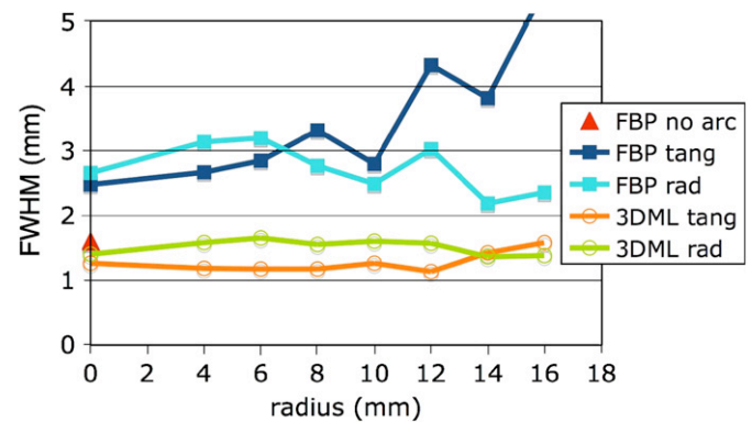
Fig. 2. Radial and tangential spatial resolution as a function of radial distance in the field of view using Filter Back Projection and 3D MLEM reconstruction methods.
