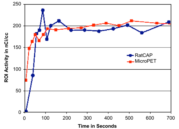
Fig. 8. Time-activity curve for a ^{11}\text{C} -methamphetamine study using the RatCAP compared to the MicroPET R4.
