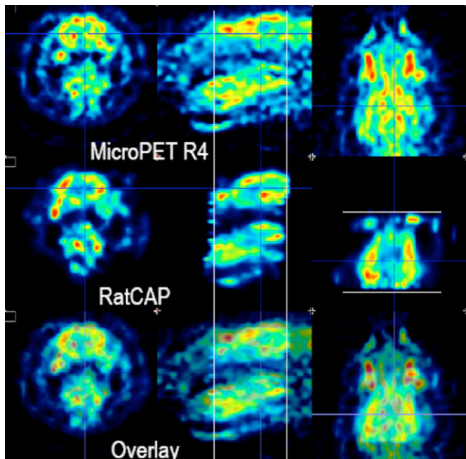
Fig. 7. ^{18}\text{F} -FDG rat brain images from the RatCAP compared to the same animal imaged with a MicroPET R4. Vertical lines show the axial coverage of the RatCAP.
